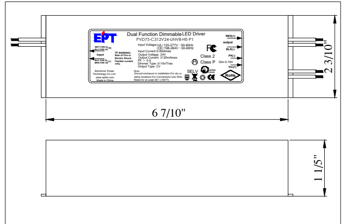
LED DRIVER DIAGRAM
