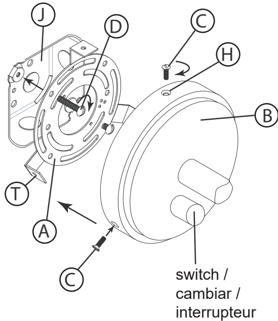
DRAWING 2 - MOUNTING
